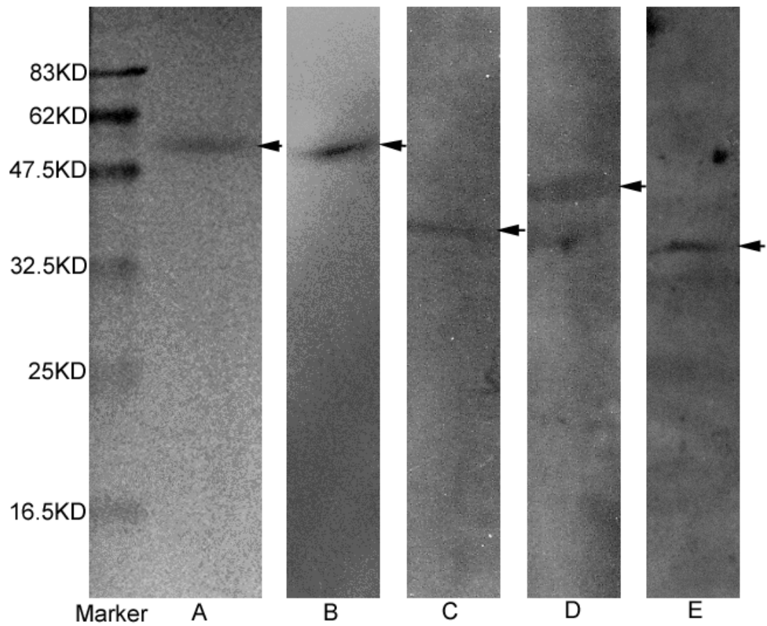
Figure 3. Western blot analysis of CCT \epsilon (A), CCT \theta (B), hnRNP E1 (C), hnRNP A2/B1 (D) and hnRNP K (E), expression in normal mouse testes.
